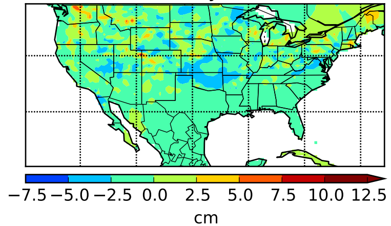
E2O Snow Analysis Increment
