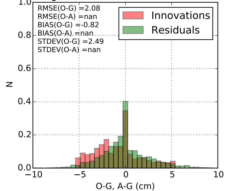
Histogram of Innovations and Residuals
