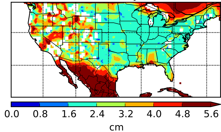
E2O Snow Analysis Error
