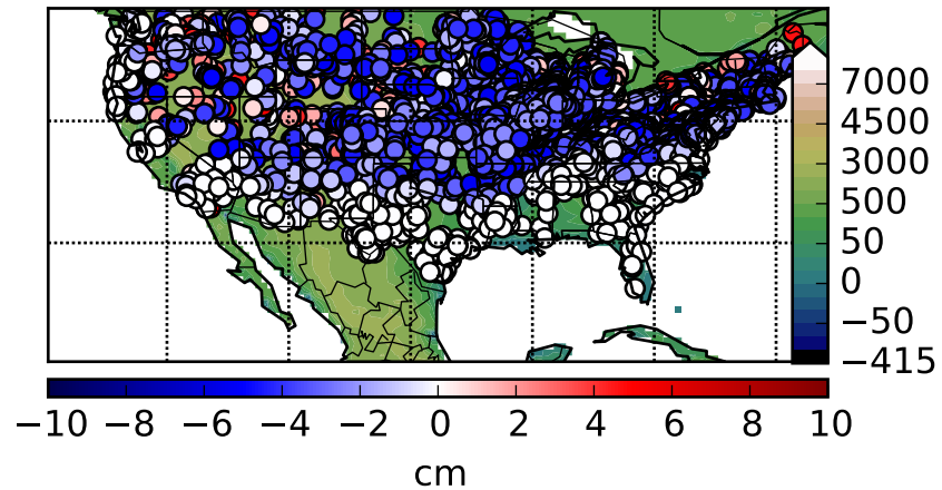
Elevation [m] and Observations locations
