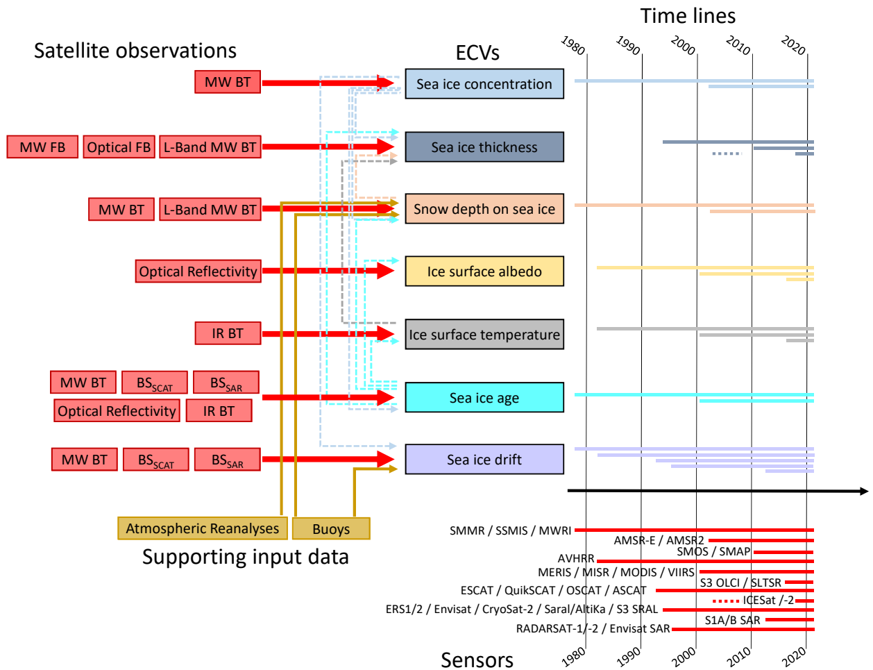
FIG. 2. Overview of the seven ECVs and their potential temporal coverage based on available satellite observations. On the left side we display input satellite observations: MW=microwave, FB=freeboard, BT=brightness temperature, BS=backscatter, IR=infrared, SCAT=scatterometer, SAR=synthetic aperture radar. The middle column denotes the ECVs with two kinds of supporting data required given at the bottom. On the right side we provide the time lines for which the derivation of CDRs and data products for these ECVs has been demonstrated. Several time lines may exist per ECV denoting CDRs derived from different satellite sensors. These sensors and their time lines (in red) we provide at the bottom right. The dotted time line for one of the sea-ice thickness products is for ICESat providing discontinuous coverage; all other products are continuous as far as allowed by their retrieval.
