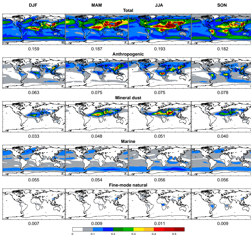
Fig. 2. Seasonal distributions of aerosol optical depth at 0.55 \mu\text{m} as derived from the MACC re-analysis over 2003–2010. From top to bottom, the optical depth is for total, anthropogenic, mineral dust, marine, and fine-mode natural aerosols. Global averages are given by the numbers below each panel.
