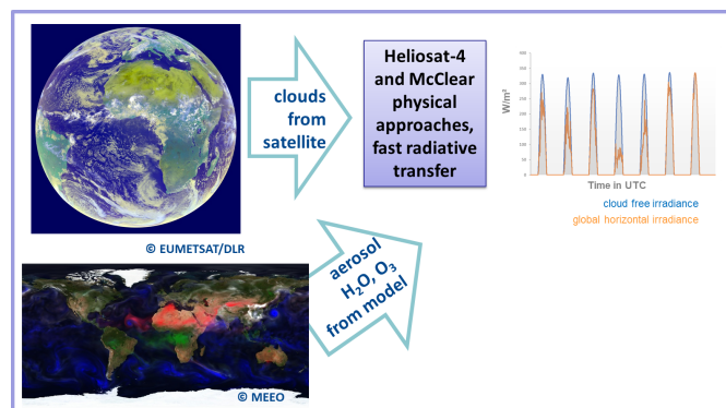
Fig. 2-2: Combination of satellite-based cloud information with model based aerosol, water vapour and ozone information to derive time series of solar radiation at the surface in cloudy and cloud-free conditions
