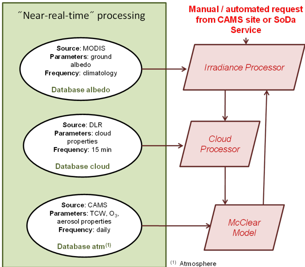
Figure 7.1. Schematic representation of the workflow of the CAMS Radiation Service for computing irradiance products.
