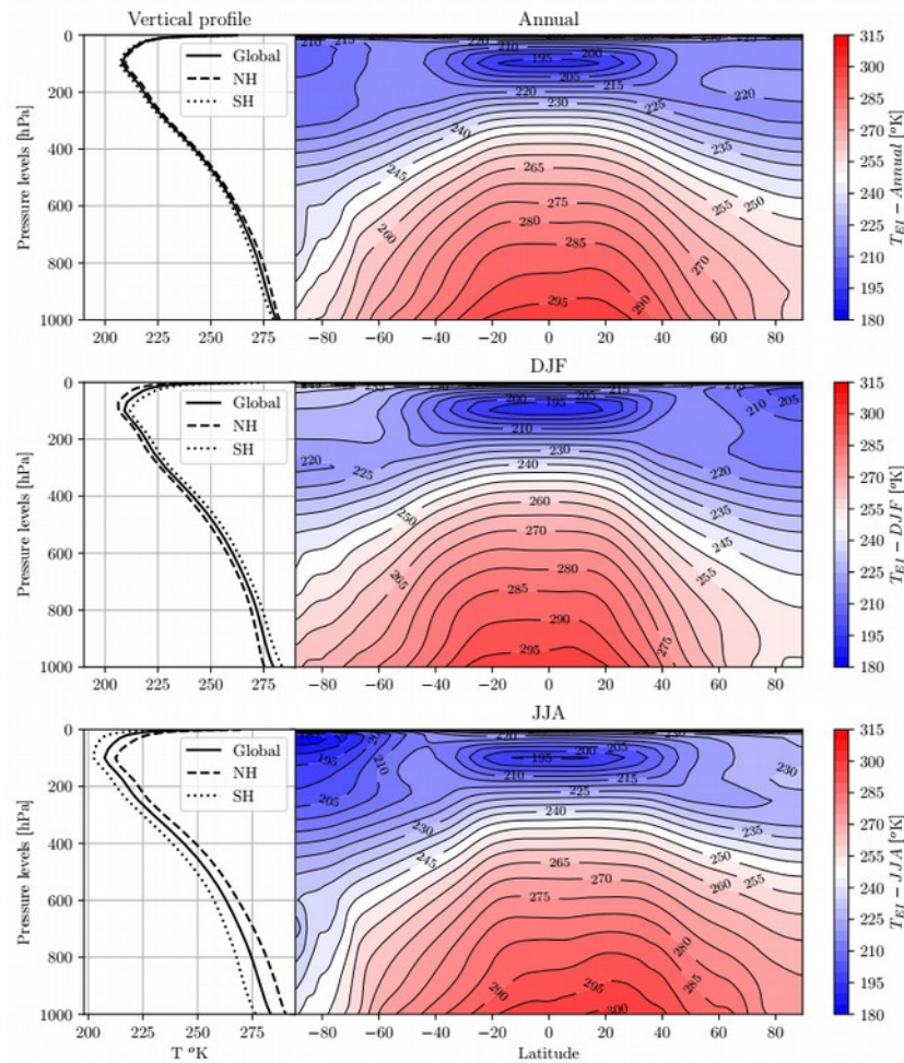
Zonal mean Temperature profile ERA-INTERIM-1979-2018
