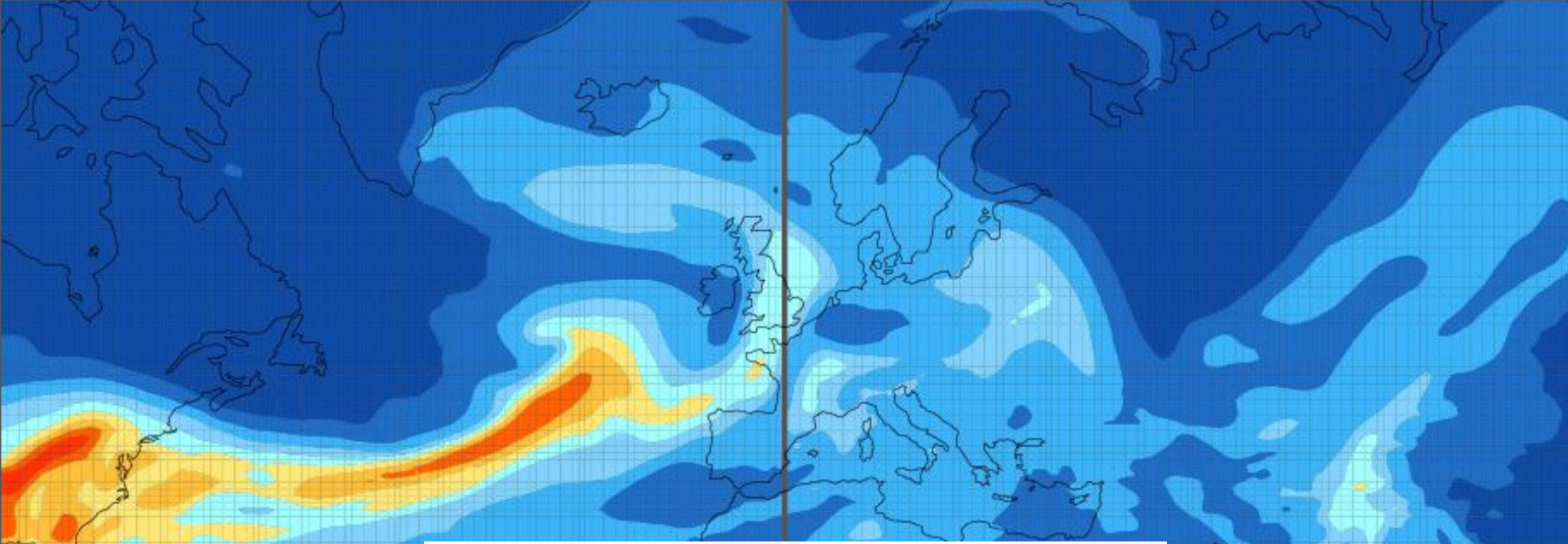
ERA-Interim Total Column Water Vapour (TCWV) 18UTC 31 Jan 2002
