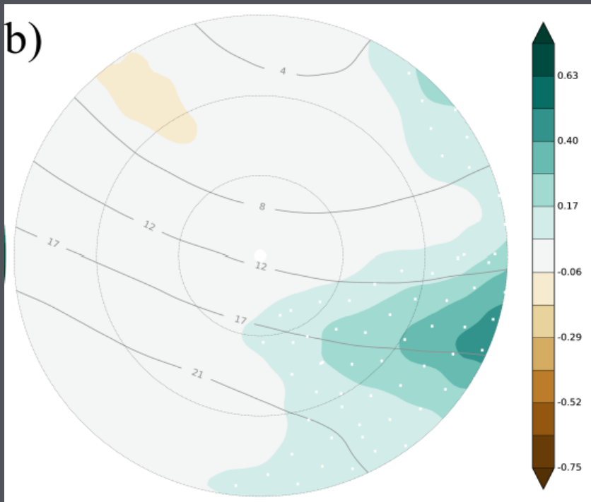
Composite 10-day filtered TCWV at T-24 (contours) and sensitivity of precipitation ( \text{kg m}^{-2} ) at max intensity to TCWV 24 hrs earlier
