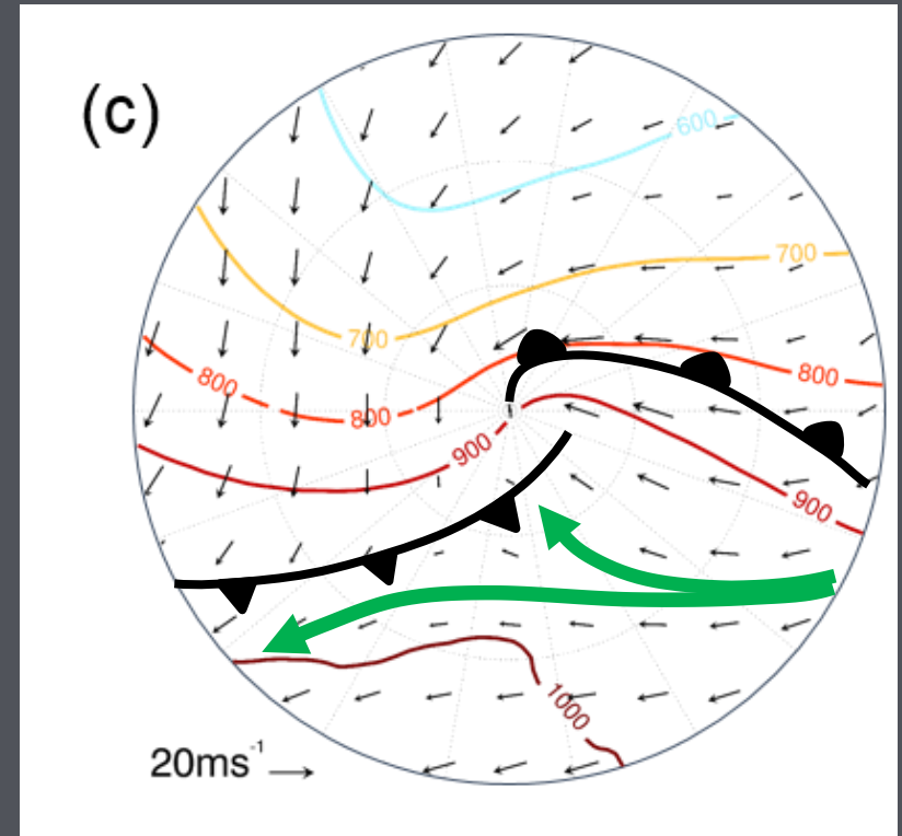
Pressure in hPa (contours) and cyclone-relative winds (vectors) on 285 K \theta surface at T-24
