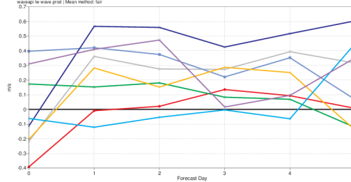
10m wind speed Mean error North Sea (lat 51.5 to 62.0, lon -1.0 to 10.0) Date: 20190301 00UTC to 20190531 12UTC wrapup: le wave prod | Mean method: tar
