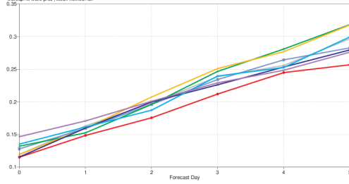
10m wind speed Scatter index North Sea (lat 51.5 to 62.0, lon -1.0 to 10.0) Date: 20190301 00UTC to 20190531 12UTC wrapup: le wave prod | Mean method: tar
