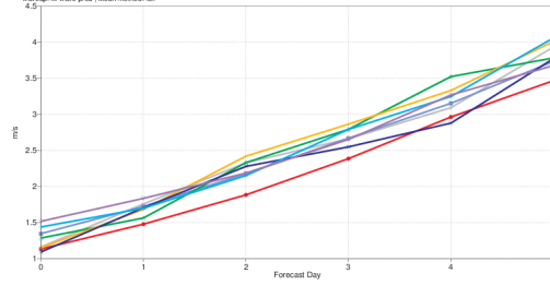
10m wind speed Root mean square error North Sea (lat 51.5 to 62.0, lon -1.0 to 10.0) Date: 20190301 00UTC to 20190531 12UTC wrapup: le wave prod | Mean method: tar
